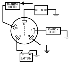
MP39830 – BLISTER PACK MP39832 – BULK 100 PCS/CTN
